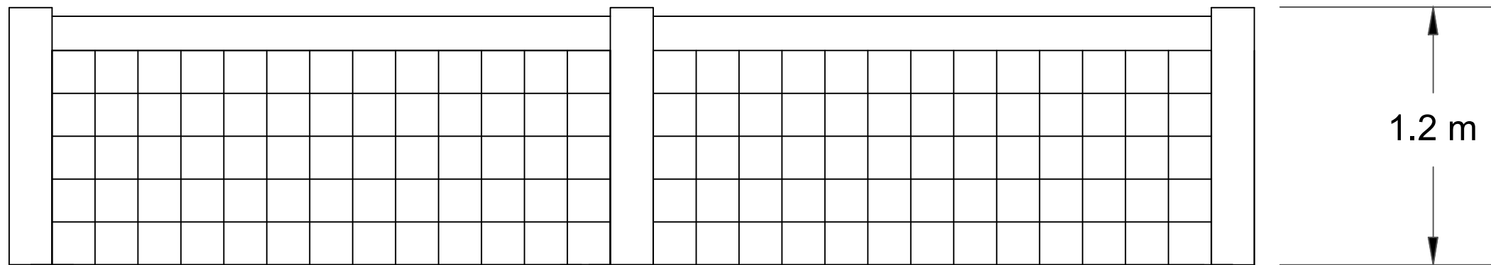
Side View
